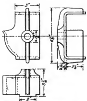
Figs. 3887-3889. Uncoupling Chain Sheave Housing.
